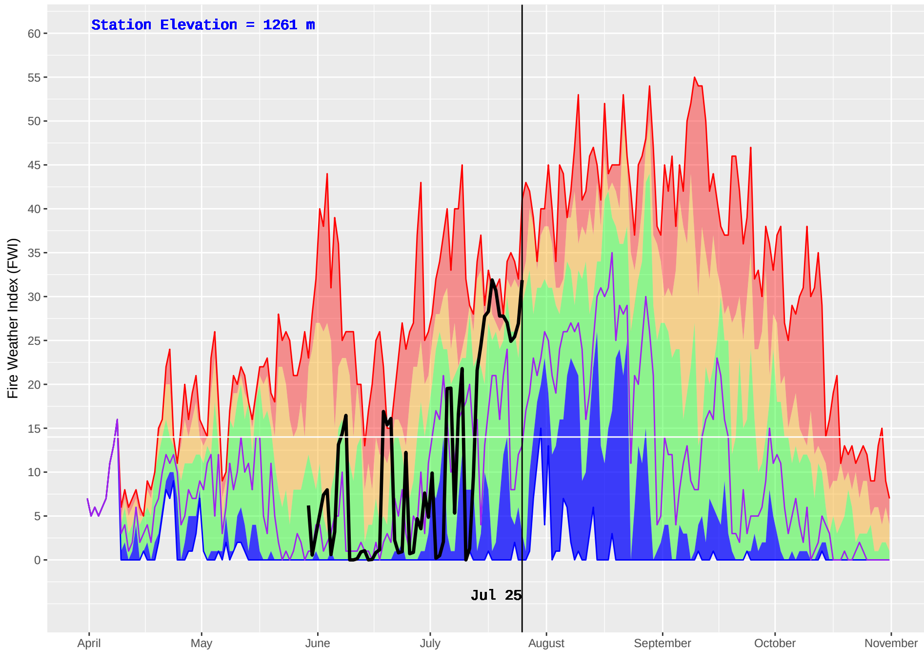
IDA BELL LAKE 3 (876) : Historical (2004–2016) and Current (2018) Noon Fire Weather Index (FWI)
