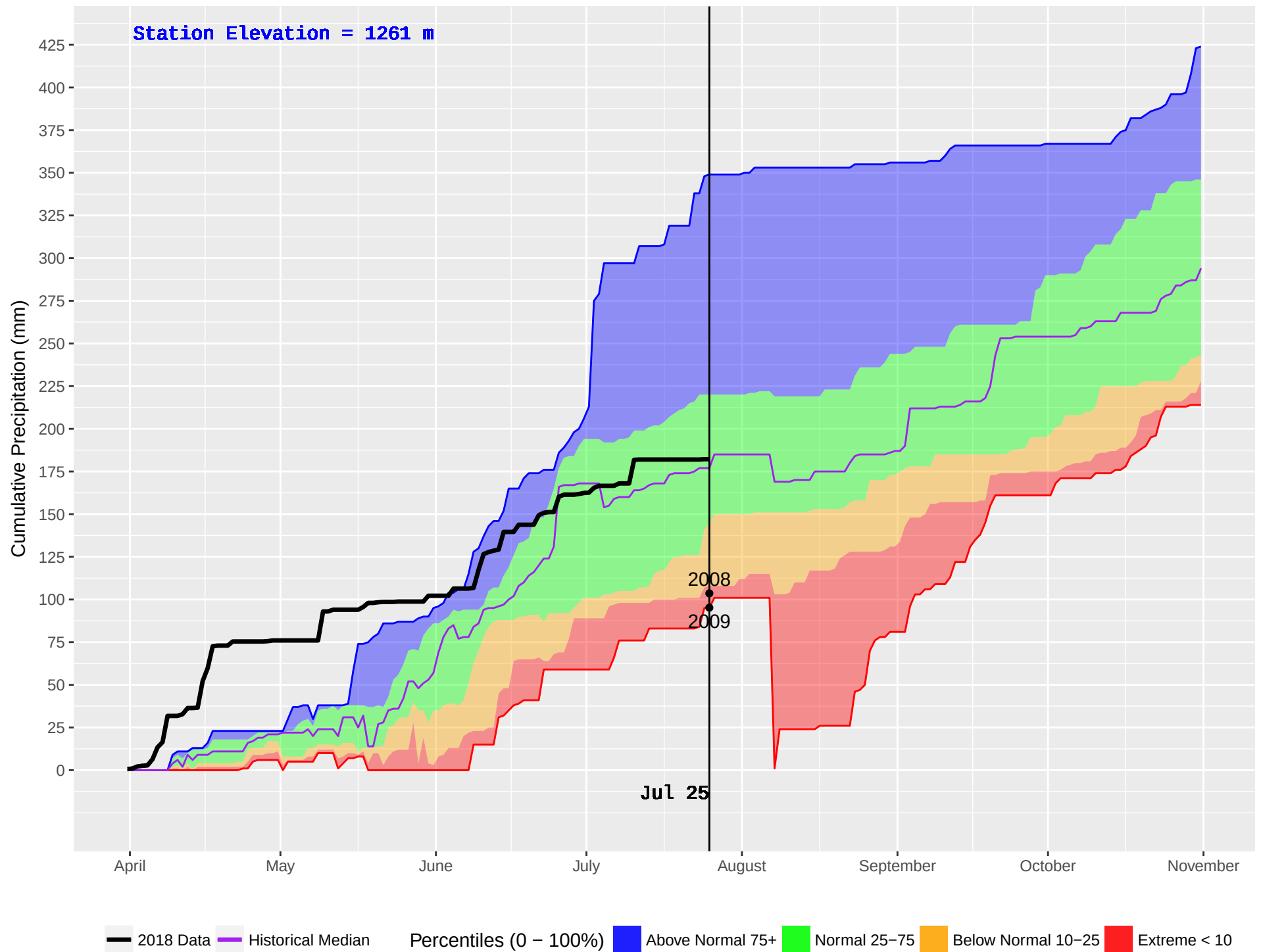
IDA BELL LAKE 3 (876) : Historical (2004–2016) and Current (2018) Noon Cumulative Precipitation
