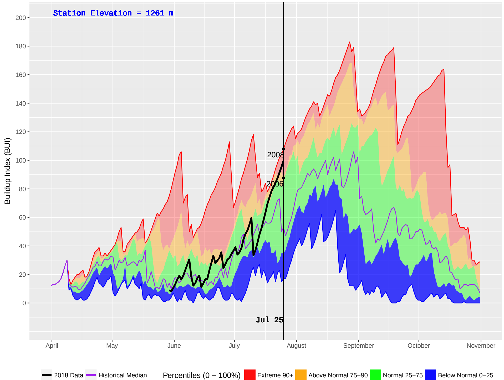
IDA BELL LAKE 3 (876) : Historical (2004–2016) and Current (2018) Noon Buildup Index (BUI)
