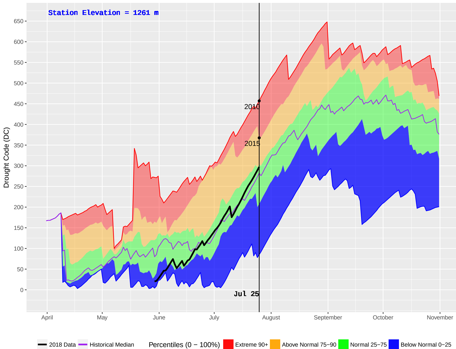
IDA BELL LAKE 3 (876) : Historical (2004–2016) and Current (2018) Noon Drought Code (DC)
